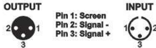
Three core canon plug DMX512 interface circuit
