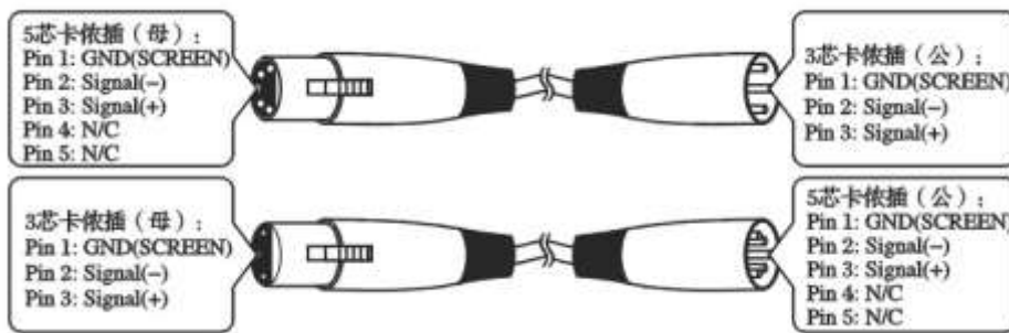
Three core canon plug DMX512 interface circuit
